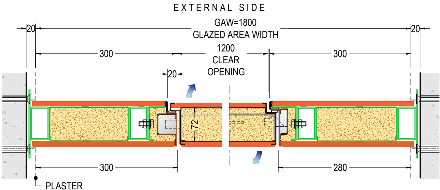
DOOR HORIZONTAL SECTION MODELS "E-F"
