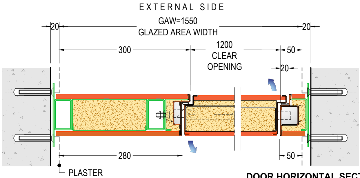
DOOR HORIZONTAL SECTION MODELS "C-G"
